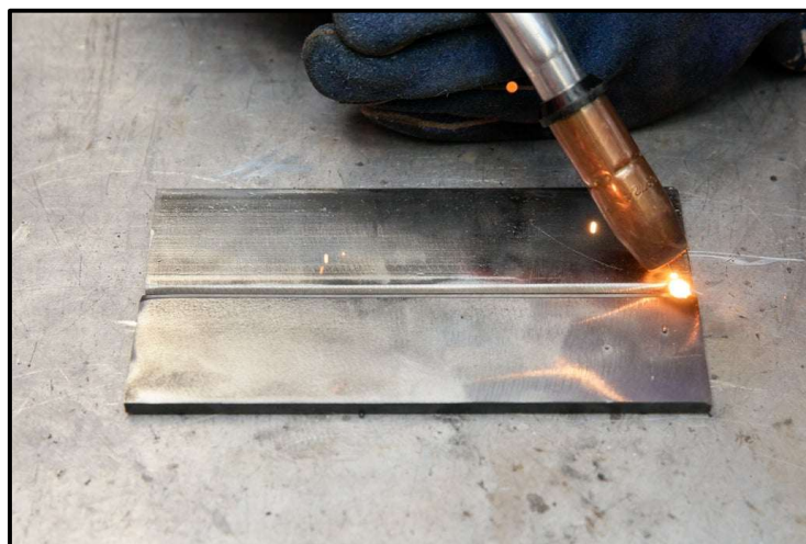
Figure 15: Tag weld
